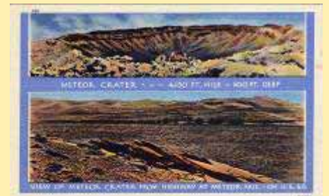
165 Meteor Crater 0 4150 Ft. Wide—600
