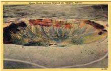
111 Meteor Crater Between Flagstaff An
