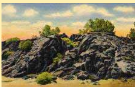
21 Volcanic Lava
